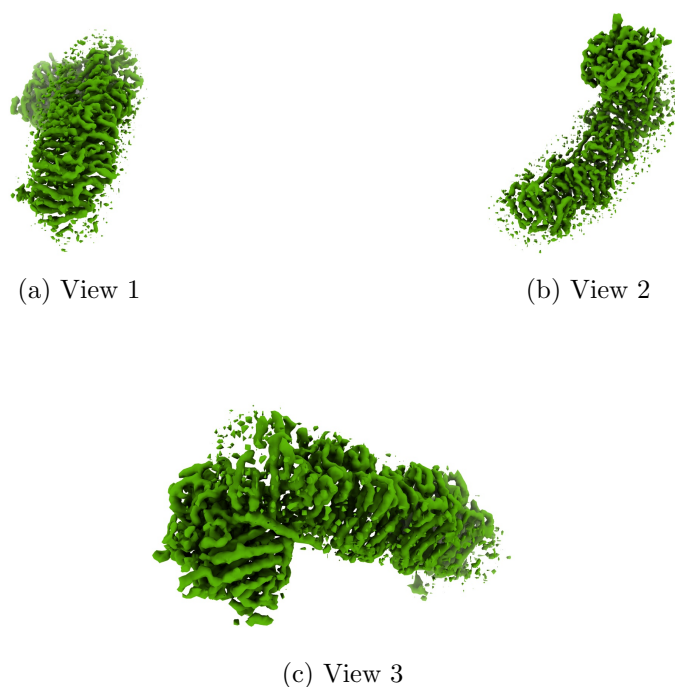
Figure 4: Isosurface at threshold=0.012600. Views generated by ChimeraX at a the following X, Y, Z angles: View 1 (0, -90, -90), View 2 (-90, 0, -90), View 3 (0, 0, 0).
