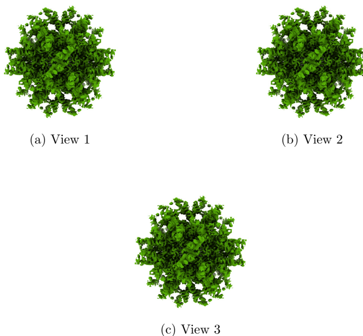
Figure 4: Isosurface at threshold=0.038500. Views generated by ChimeraX at a the following X, Y, Z angles: View 1 (0, -90, -90), View 2 (-90, 0, -90), View 3 (0, 0, 0).
