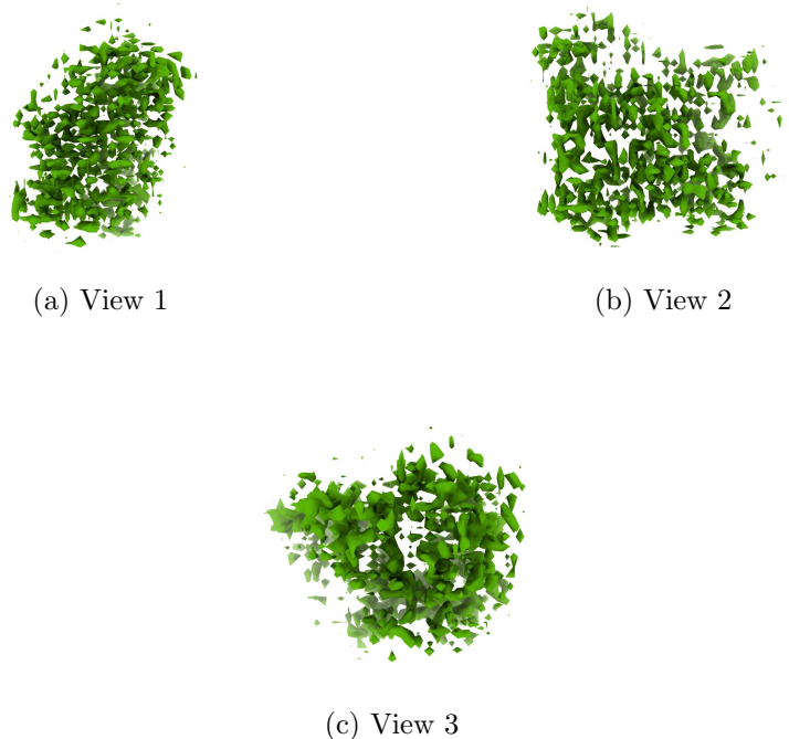
Figure 4: Isosurface at threshold=0.080000. Views generated by ChimeraX at a the following X, Y, Z angles: View 1 (0, -90, -90), View 2 (-90, 0, -90), View 3 (0, 0, 0).
