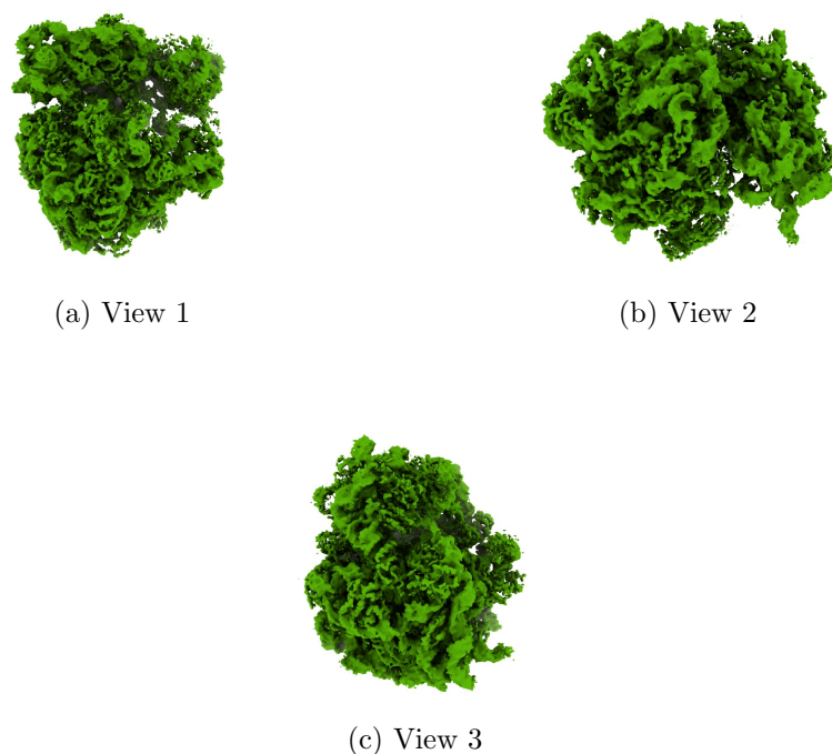
Figure 4: Isosurface at threshold=0.022200. Views generated by ChimeraX at a the following X, Y, Z angles: View 1 (0, -90, -90), View 2 (-90, 0, -90), View 3 (0, 0, 0).
