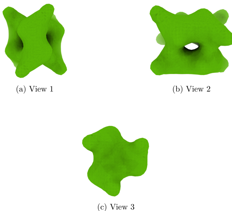
Figure 4: Isosurface at threshold=11.100000. Views generated by ChimeraX at a the following X, Y, Z angles: View 1 (0, -90, -90), View 2 (-90, 0, -90), View 3 (0, 0, 0).
