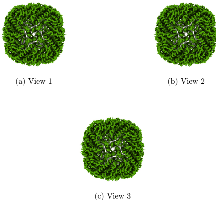
Figure 4: Isosurface at threshold=0.031800. Views generated by ChimeraX at a the following X, Y, Z angles: View 1 (0, -90, -90), View 2 (-90, 0, -90), View 3 (0, 0, 0).
