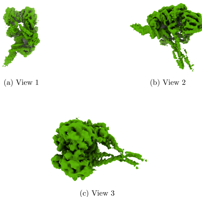
Figure 4: Isosurface at threshold=0.009100. Views generated by ChimeraX at a the following X, Y, Z angles: View 1 (0, -90, -90), View 2 (-90, 0, -90), View 3 (0, 0, 0).
