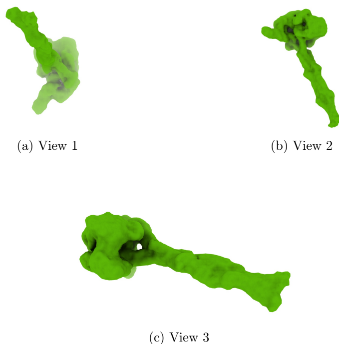
Figure 4: Isosurface at threshold=0.030400. Views generated by ChimeraX at a the following X, Y, Z angles: View 1 (0, -90, -90), View 2 (-90, 0, -90), View 3 (0, 0, 0).
