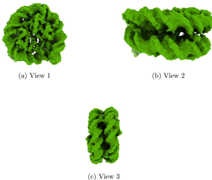
Figure 4: Isosurface at threshold=0.009400. Views generated by ChimeraX at a the following X, Y, Z angles: View 1 (0, -90, -90), View 2 (-90, 0, -90), View 3 (0, 0, 0).
