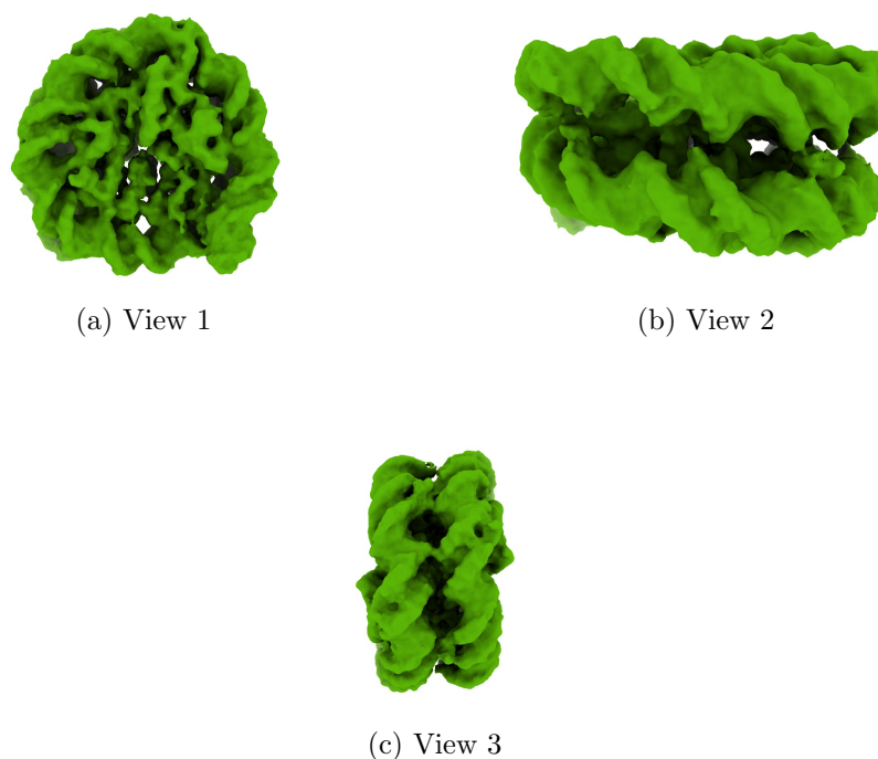
Figure 4: Isosurface at threshold=0.009200. Views generated by ChimeraX at a the following X, Y, Z angles: View 1 (0, -90, -90), View 2 (-90, 0, -90), View 3 (0, 0, 0).
