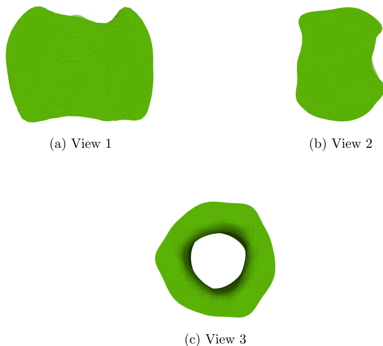
Figure 4: Isosurface at threshold=7.220000. Views generated by ChimeraX at a the following X, Y, Z angles: View 1 (0, -90, -90), View 2 (-90, 0, -90), View 3 (0, 0, 0).
