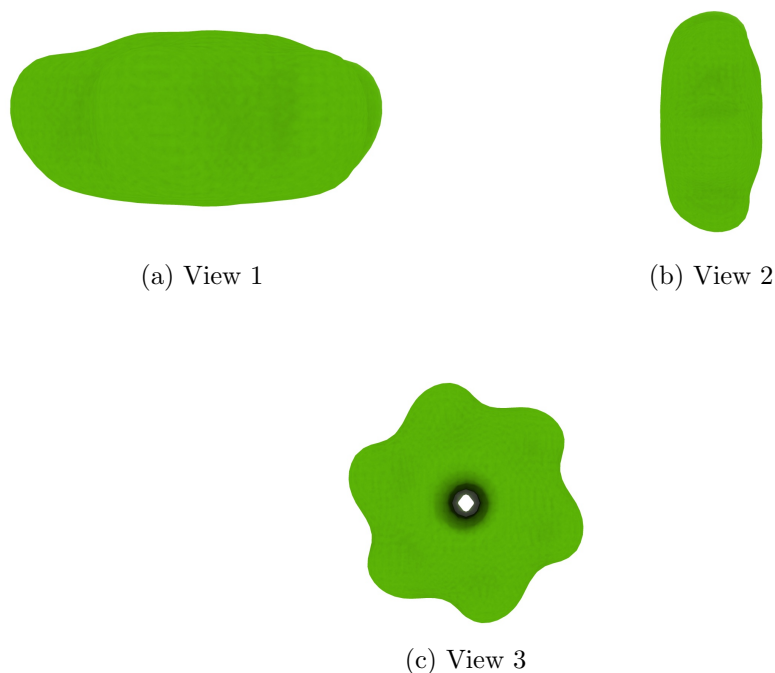
Figure 4: Isosurface at threshold=11.500000. Views generated by ChimeraX at a the following X, Y, Z angles: View 1 (0, -90, -90), View 2 (-90, 0, -90), View 3 (0, 0, 0).
