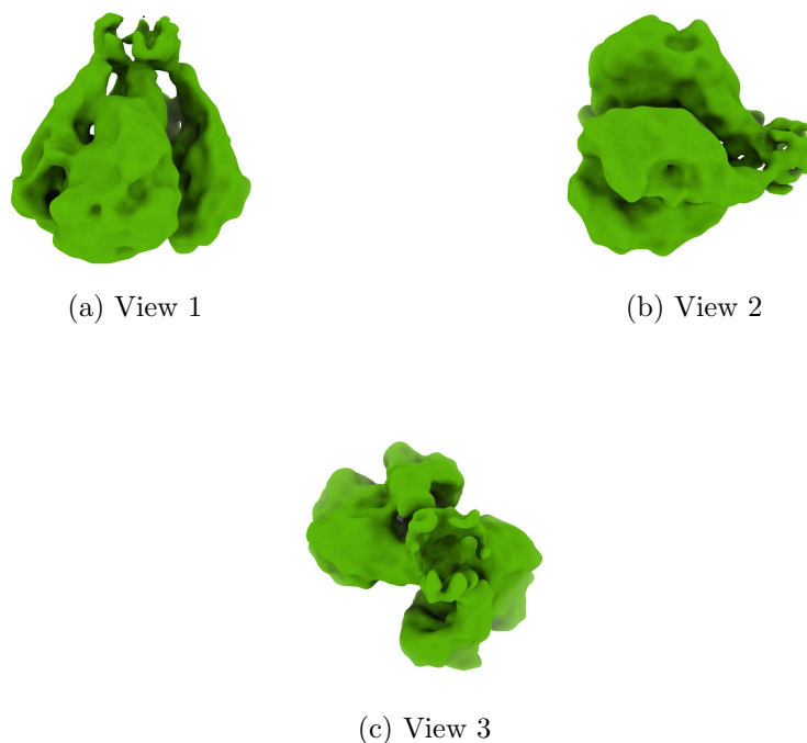
Figure 4: Isosurface at threshold=0.006500. Views generated by ChimeraX at a the following X, Y, Z angles: View 1 (0, -90, -90), View 2 (-90, 0, -90), View 3 (0, 0, 0).
