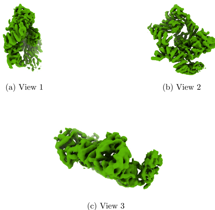
Figure 4: Isosurface at threshold=0.012800. Views generated by ChimeraX at a the following X, Y, Z angles: View 1 (0, -90, -90), View 2 (-90, 0, -90), View 3 (0, 0, 0).
