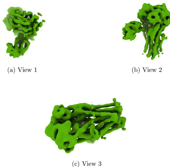
Figure 4: Isosurface at threshold=0.013300. Views generated by ChimeraX at a the following X, Y, Z angles: View 1 (0, -90, -90), View 2 (-90, 0, -90), View 3 (0, 0, 0).
