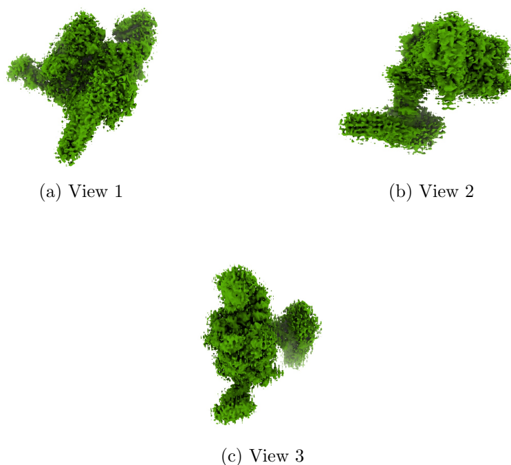
Figure 4: Isosurface at threshold=0.013500. Views generated by ChimeraX at a the following X, Y, Z angles: View 1 (0, -90, -90), View 2 (-90, 0, -90), View 3 (0, 0, 0).
