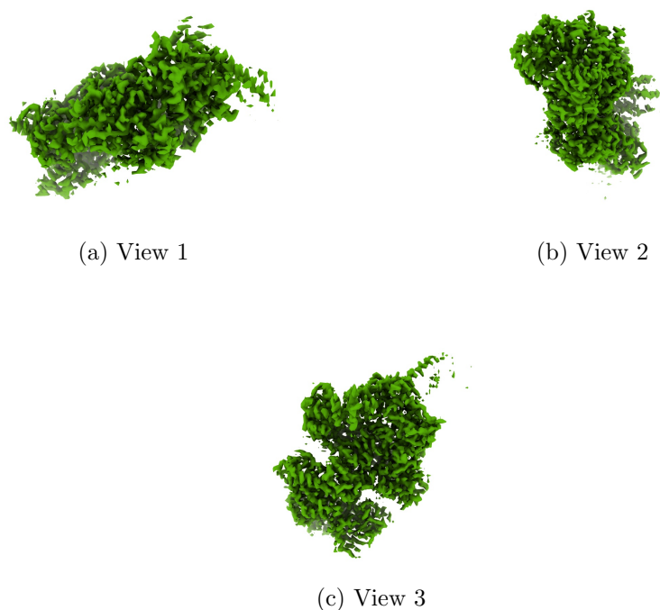
Figure 4: Isosurface at threshold=0.040300. Views generated by ChimeraX at a the following X, Y, Z angles: View 1 (0, -90, -90), View 2 (-90, 0, -90), View 3 (0, 0, 0).
