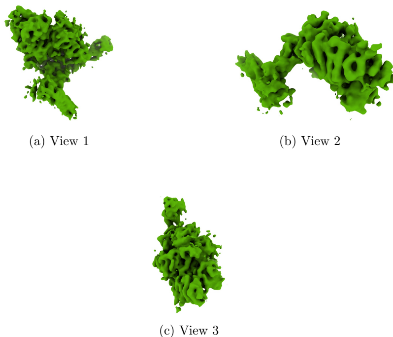
Figure 4: Isosurface at threshold=0.049000. Views generated by ChimeraX at a the following X, Y, Z angles: View 1 (0, -90, -90), View 2 (-90, 0, -90), View 3 (0, 0, 0).
