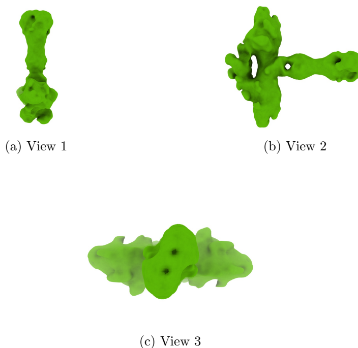
Figure 4: Isosurface at threshold=0.072800. Views generated by ChimeraX at a the following X, Y, Z angles: View 1 (0, -90, -90), View 2 (-90, 0, -90), View 3 (0, 0, 0).
