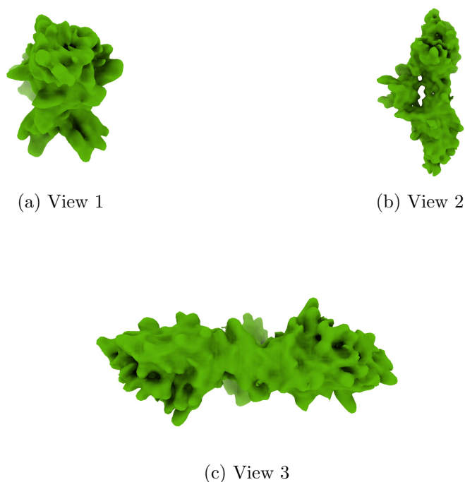
Figure 4: Isosurface at threshold=0.128000. Views generated by ChimeraX at a the following X, Y, Z angles: View 1 (0, -90, -90), View 2 (-90, 0, -90), View 3 (0, 0, 0).
