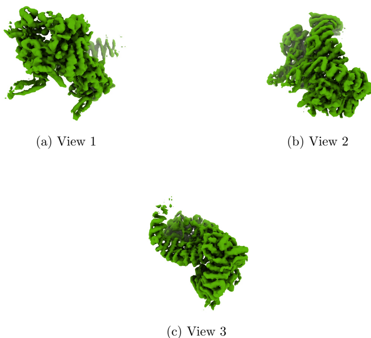
Figure 4: Isosurface at threshold=0.380000. Views generated by ChimeraX at a the following X, Y, Z angles: View 1 (0, -90, -90), View 2 (-90, 0, -90), View 3 (0, 0, 0).
