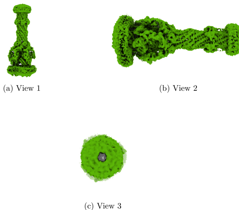
Figure 4: Isosurface at threshold=0.012500. Views generated by ChimeraX at a the following X, Y, Z angles: View 1 (0, -90, -90), View 2 (-90, 0, -90), View 3 (0, 0, 0).
