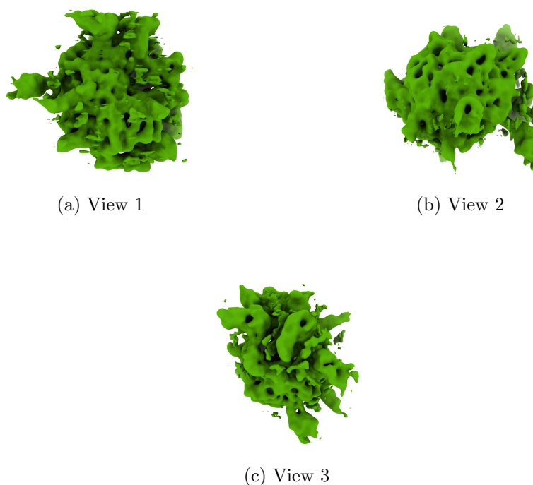
Figure 4: Isosurface at threshold=0.010800. Views generated by ChimeraX at a the following X, Y, Z angles: View 1 (0, -90, -90), View 2 (-90, 0, -90), View 3 (0, 0, 0).
