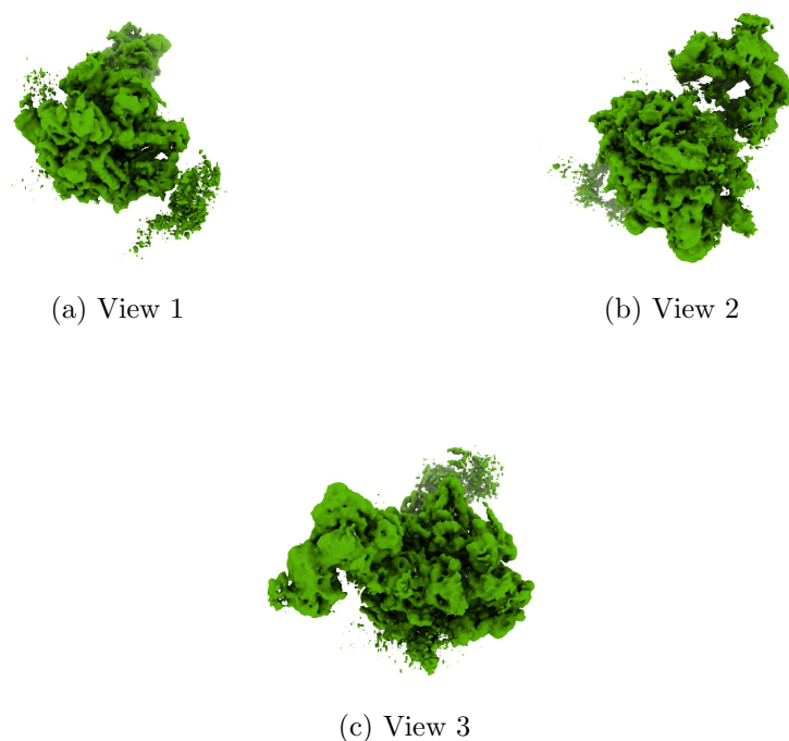
Figure 4: Isosurface at threshold=0.015500. Views generated by ChimeraX at a the following X, Y, Z angles: View 1 (0, -90, -90), View 2 (-90, 0, -90), View 3 (0, 0, 0).
