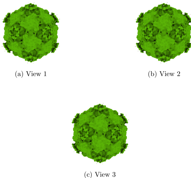
Figure 4: Isosurface at threshold=4380.000000. Views generated by ChimeraX at the following X, Y, Z angles: View 1 (0, -90, -90), View 2 (-90, 0, -90), View 3 (0, 0, 0).
