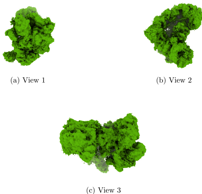
Figure 4: Isosurface at threshold=0.004850. Views generated by ChimeraX at a the following X, Y, Z angles: View 1 (0, -90, -90), View 2 (-90, 0, -90), View 3 (0, 0, 0).
