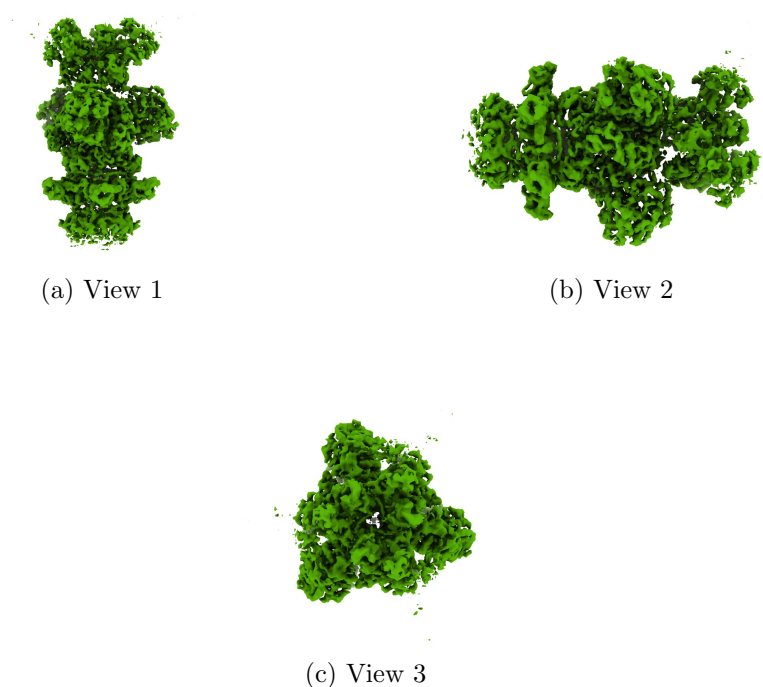
Figure 4: Isosurface at threshold=0.055700. Views generated by ChimeraX at a the following X, Y, Z angles: View 1 (0, -90, -90), View 2 (-90, 0, -90), View 3 (0, 0, 0).
