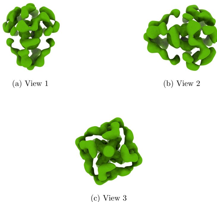
Figure 4: Isosurface at threshold=0.063700. Views generated by ChimeraX at a the following X, Y, Z angles: View 1 (0, -90, -90), View 2 (-90, 0, -90), View 3 (0, 0, 0).
