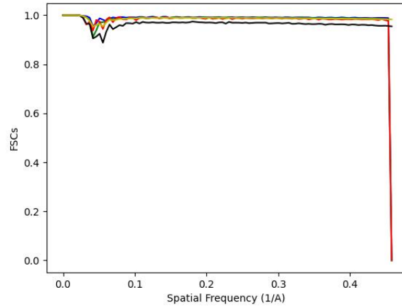
Figure 28: FSC in X, Y, Z, the global FSC, and the Average Cosine Phase.
