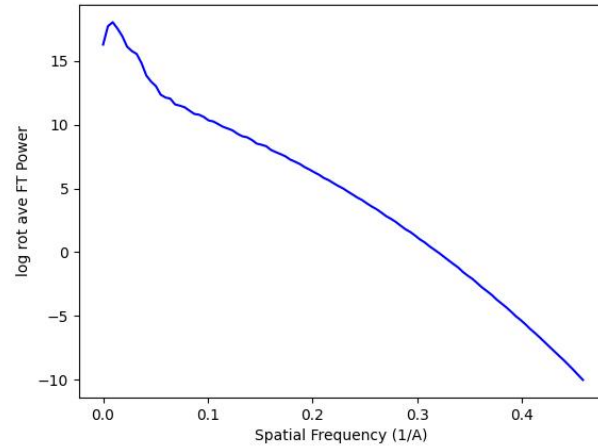
Figure 30: Logarithm of the radial average of the input map power in Fourier space.
