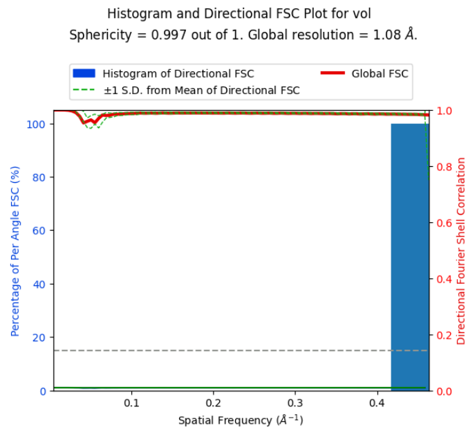
Figure 29: Global FSC and histogram of the directional FSC.
