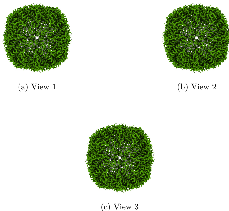
Figure 4: Isosurface at threshold=0.057600. Views generated by ChimeraX at the following X, Y, Z angles: View 1 (0, -90, -90), View 2 (-90, 0, -90), View 3 (0, 0, 0).
