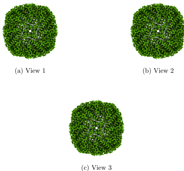
Figure 4: Isosurface at threshold=0.051100. Views generated by ChimeraX at a the following X, Y, Z angles: View 1 (0, -90, -90), View 2 (-90, 0, -90), View 3 (0, 0, 0).
