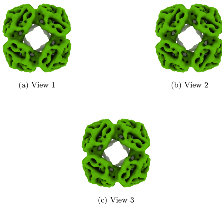
Figure 4: Isosurface at threshold=0.085700. Views generated by ChimeraX at a the following X, Y, Z angles: View 1 (0, -90, -90), View 2 (-90, 0, -90), View 3 (0, 0, 0).
