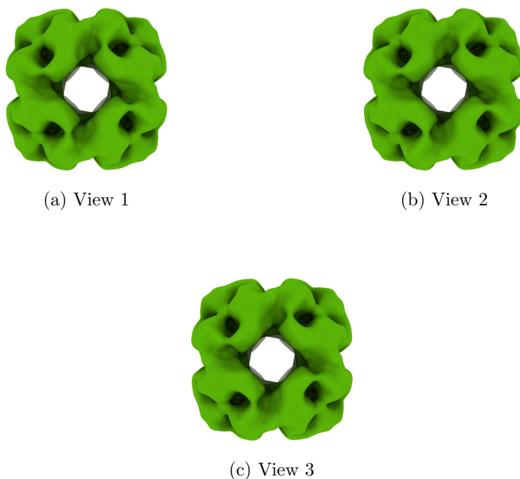
Figure 4: Isosurface at threshold=0.037500. Views generated by ChimeraX at a the following X, Y, Z angles: View 1 (0, -90, -90), View 2 (-90, 0, -90), View 3 (0, 0, 0).
