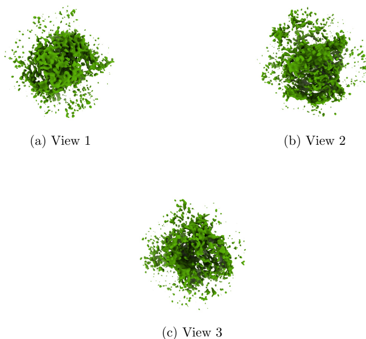
Figure 4: Isosurface at threshold=65.200000. Views generated by ChimeraX at a the following X, Y, Z angles: View 1 (0, -90, -90), View 2 (-90, 0, -90), View 3 (0, 0, 0).
