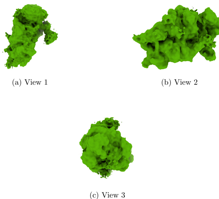
Figure 4: Isosurface at threshold=0.069700. Views generated by ChimeraX at a the following X, Y, Z angles: View 1 (0, -90, -90), View 2 (-90, 0, -90), View 3 (0, 0, 0).
