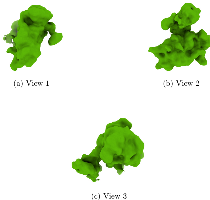
Figure 4: Isosurface at threshold=0.069200. Views generated by ChimeraX at a the following X, Y, Z angles: View 1 (0, -90, -90), View 2 (-90, 0, -90), View 3 (0, 0, 0).
