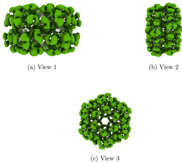
Figure 4: Isosurface at threshold=0.559000. Views generated by ChimeraX at a the following X, Y, Z angles: View 1 (0, -90, -90), View 2 (-90, 0, -90), View 3 (0, 0, 0).
