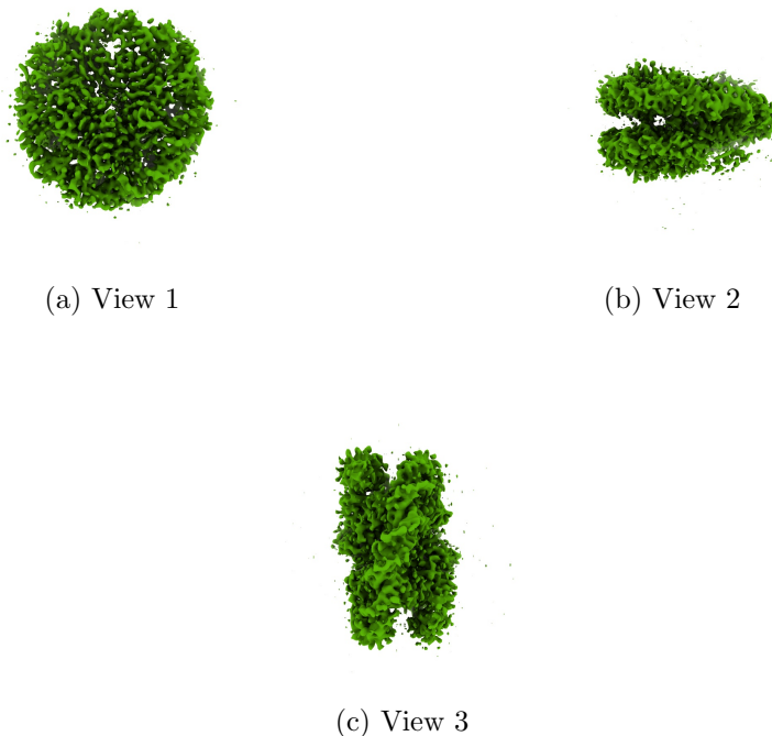
Figure 4: Isosurface at threshold=0.073500. Views generated by ChimeraX at a the following X, Y, Z angles: View 1 (0, -90, -90), View 2 (-90, 0, -90), View 3 (0, 0, 0).
