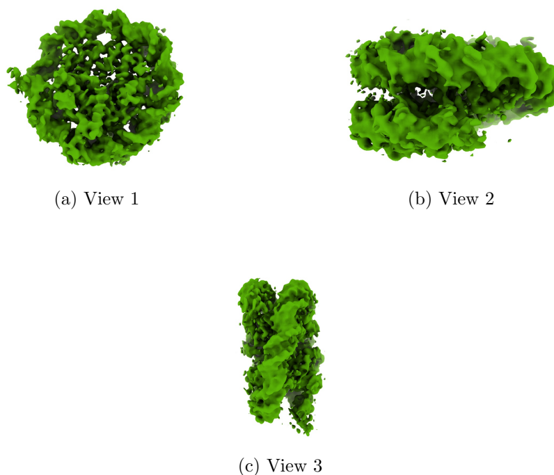
Figure 4: Isosurface at threshold=0.019300. Views generated by ChimeraX at a the following X, Y, Z angles: View 1 (0, -90, -90), View 2 (-90, 0, -90), View 3 (0, 0, 0).
