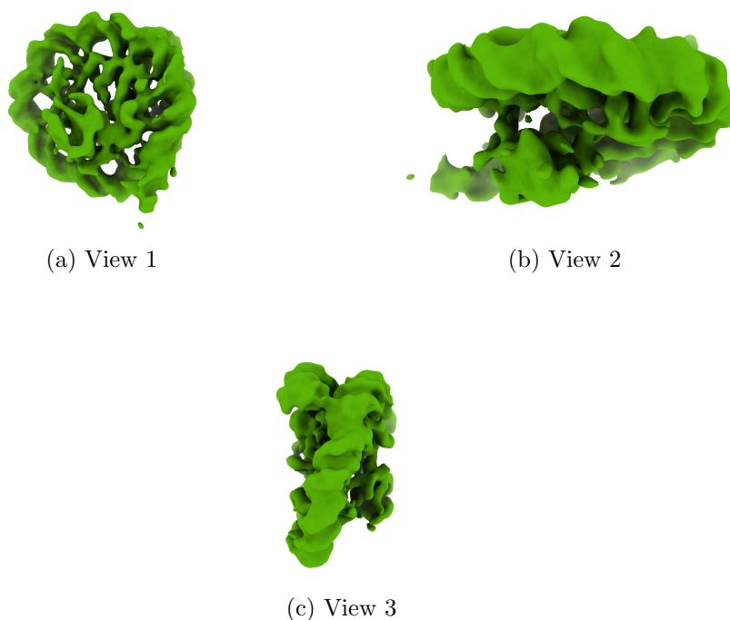
Figure 4: Isosurface at threshold=0.014380. Views generated by ChimeraX at a the following X, Y, Z angles: View 1 (0, -90, -90), View 2 (-90, 0, -90), View 3 (0, 0, 0).
