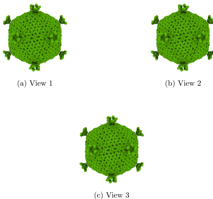
Figure 4: Isosurface at threshold=1190.000000. Views generated by ChimeraX at the following X, Y, Z angles: View 1 (0, -90, -90), View 2 (-90, 0, -90), View 3 (0, 0, 0).
