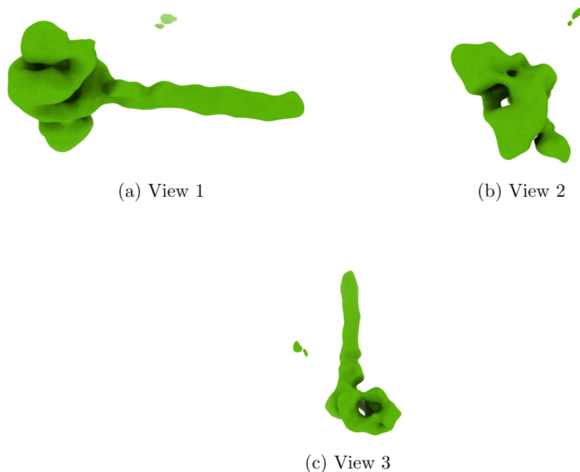
Figure 4: Isosurface at threshold=0.012500. Views generated by ChimeraX at a the following X, Y, Z angles: View 1 (0, -90, -90), View 2 (-90, 0, -90), View 3 (0, 0, 0).
