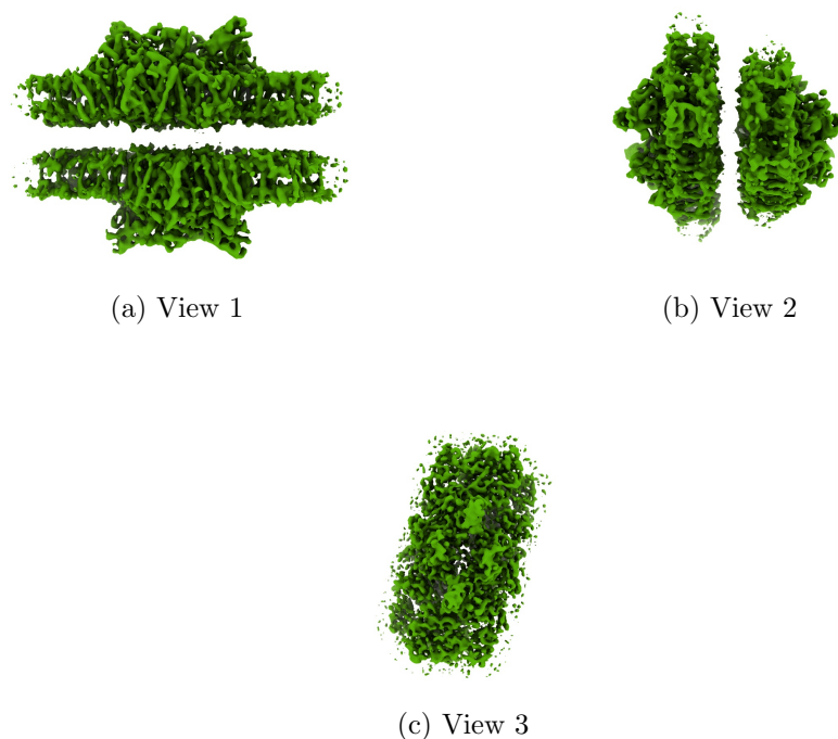
Figure 4: Isosurface at threshold=0.005630. Views generated by ChimeraX at a the following X, Y, Z angles: View 1 (0, -90, -90), View 2 (-90, 0, -90), View 3 (0, 0, 0).
