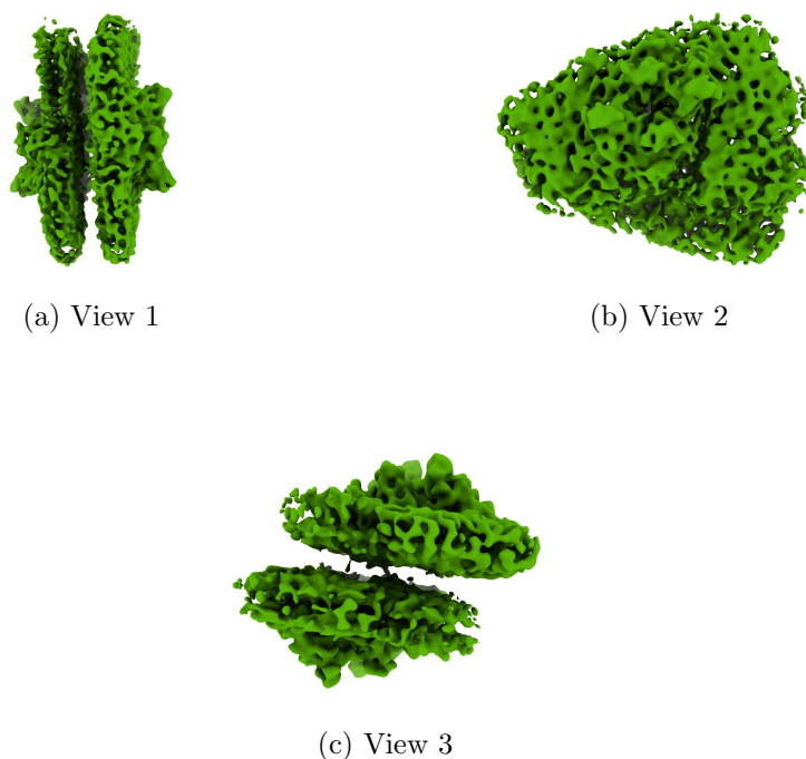
Figure 4: Isosurface at threshold=0.045200. Views generated by ChimeraX at a the following X, Y, Z angles: View 1 (0, -90, -90), View 2 (-90, 0, -90), View 3 (0, 0, 0).
