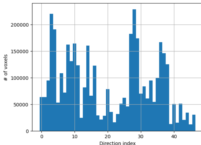
Figure 31: Histogram 1D of the best direction at each voxel.
