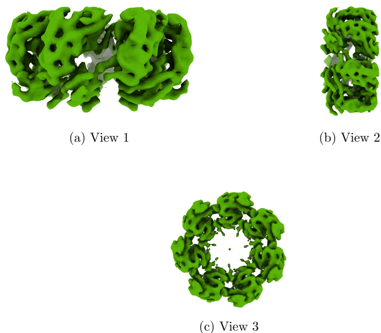
Figure 4: Isosurface at threshold=0.078000. Views generated by ChimeraX at a the following X, Y, Z angles: View 1 (0, -90, -90), View 2 (-90, 0, -90), View 3 (0, 0, 0).
