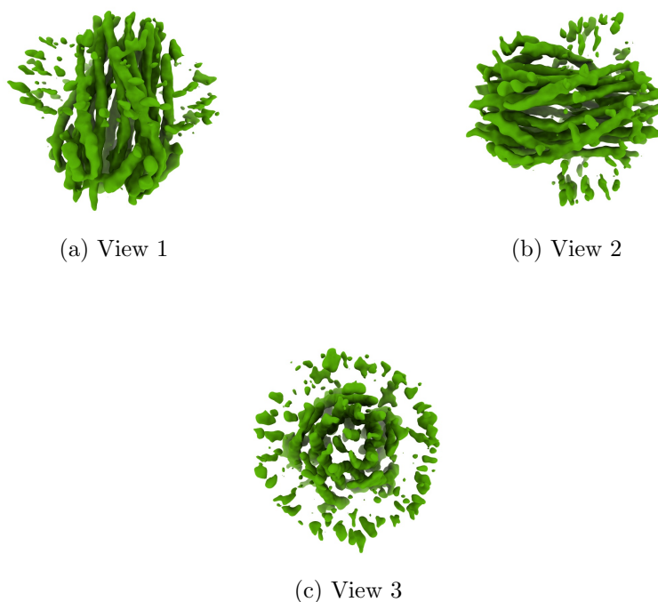
Figure 4: Isosurface at threshold=0.012800. Views generated by ChimeraX at a the following X, Y, Z angles: View 1 (0, -90, -90), View 2 (-90, 0, -90), View 3 (0, 0, 0).
