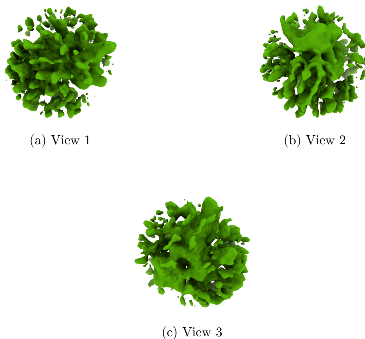
Figure 4: Isosurface at threshold=0.000084. Views generated by ChimeraX at a the following X, Y, Z angles: View 1 (0, -90, -90), View 2 (-90, 0, -90), View 3 (0, 0, 0).
