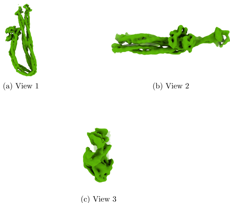
Figure 4: Isosurface at threshold=0.014500. Views generated by ChimeraX at a the following X, Y, Z angles: View 1 (0, -90, -90), View 2 (-90, 0, -90), View 3 (0, 0, 0).
