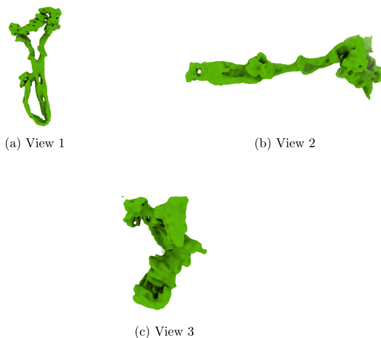
Figure 4: Isosurface at threshold=0.044400. Views generated by ChimeraX at a the following X, Y, Z angles: View 1 (0, -90, -90), View 2 (-90, 0, -90), View 3 (0, 0, 0).
